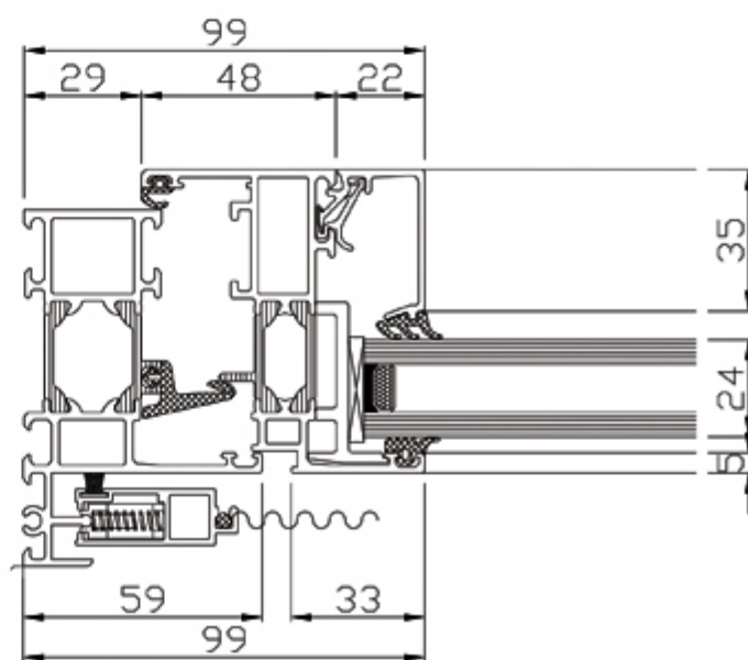
<< HORIZONTAL SECTION B-B' >>
