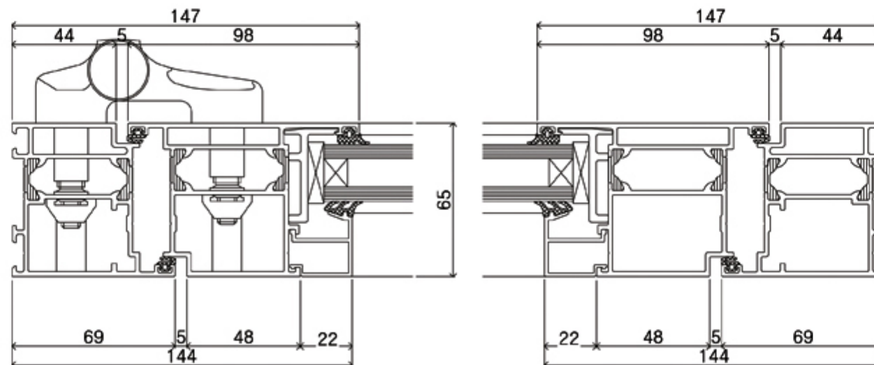
HORIZONTAL SECTION (B-B')
