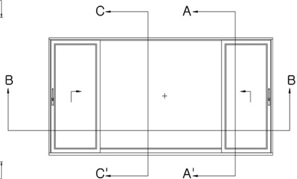
Lift Sliding Elevation
