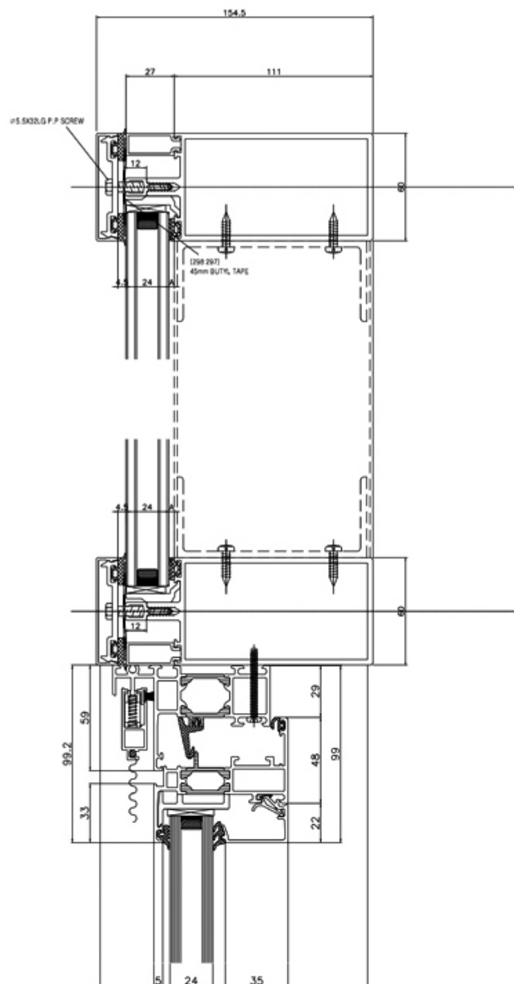
VERTICAL SECTION (A-A')
