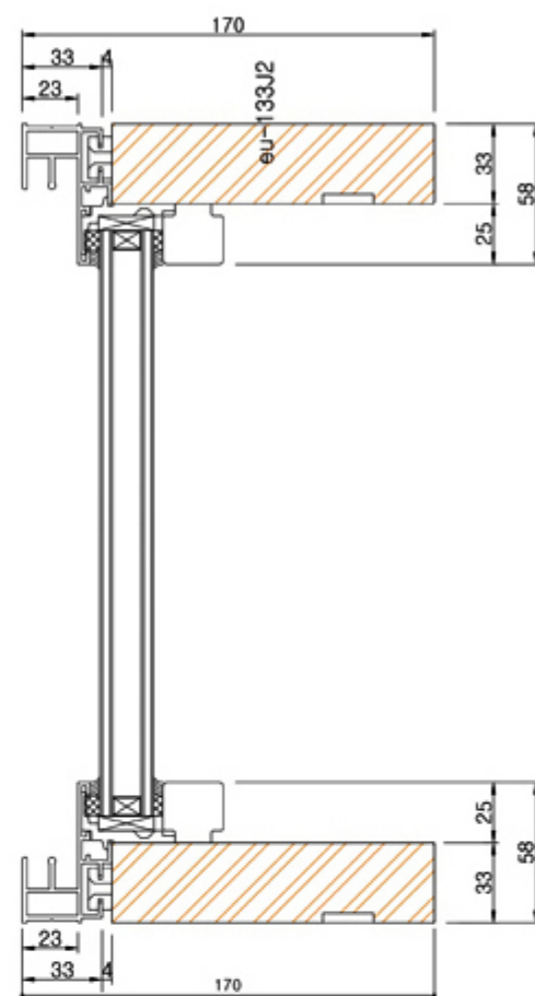
HORIZONTAL SECTION (C-C')
