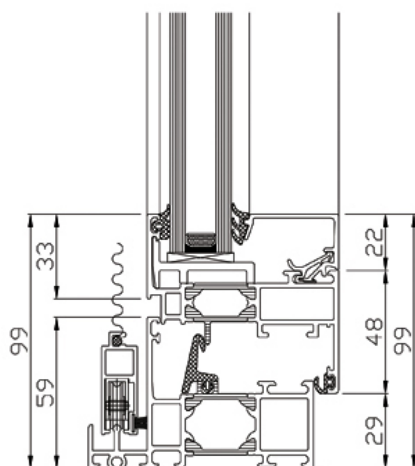
<< VERTICAL SECTION A-A' >>
