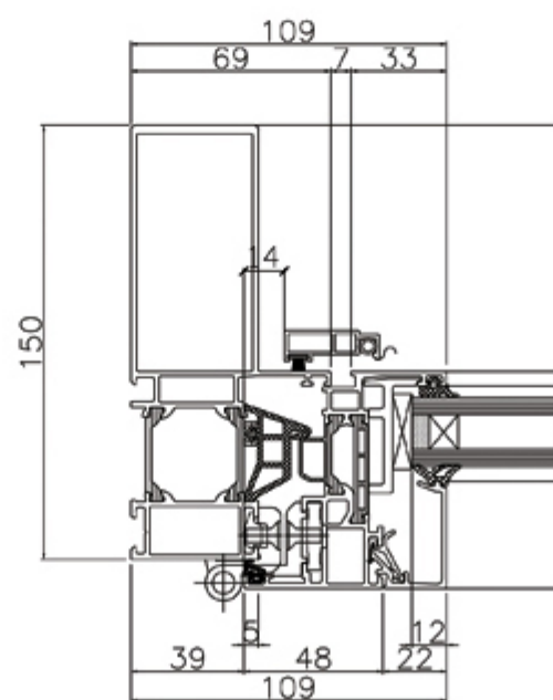
VERTICAL SECTION (A-A')
