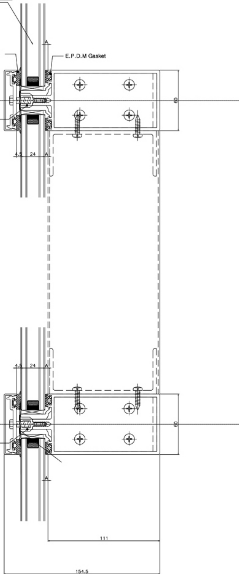
VERTICAL SECTION (A-A')
