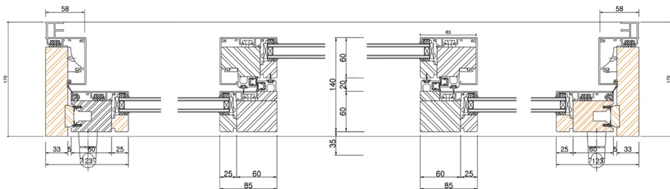
VERTICAL SECTION (B-B')
