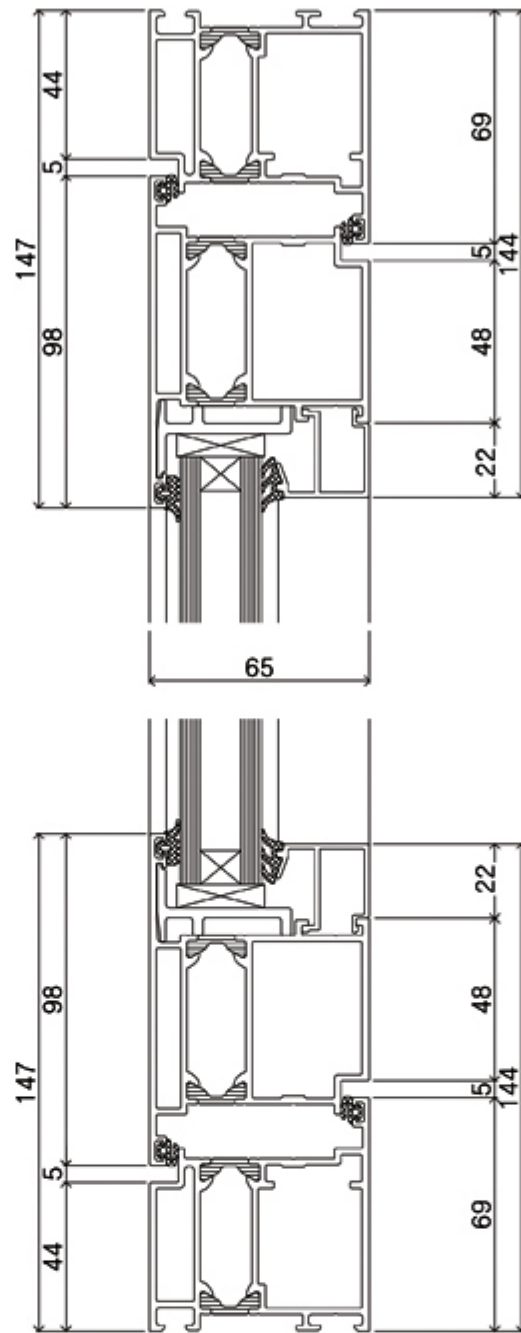
VERTICAL SECTION (A-A')
