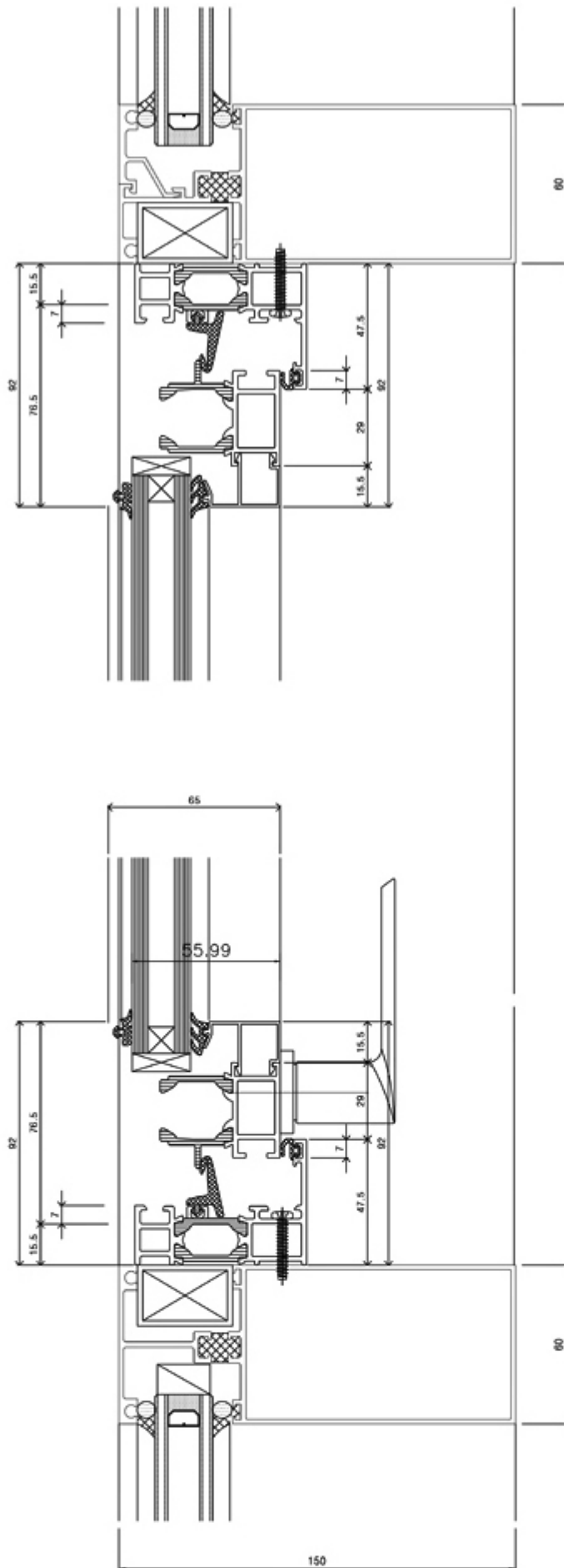
VERTICAL SECTION (A-A')
