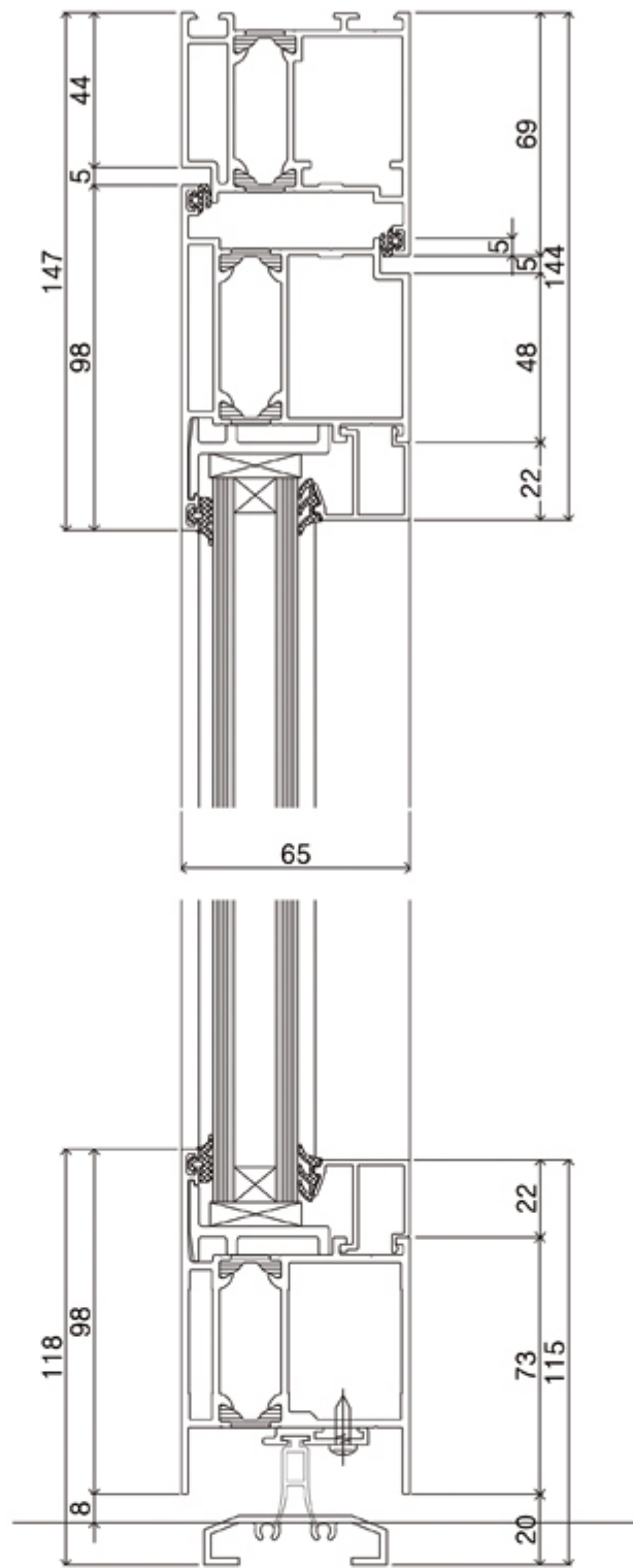
VERTICAL SECTION (A-A')
