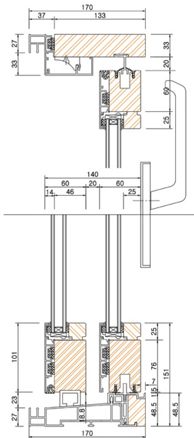
VERTICAL SECTION (A-A')
