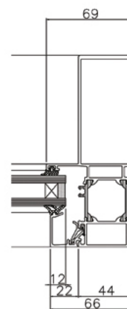
VERTICAL SECTION (B-B')
