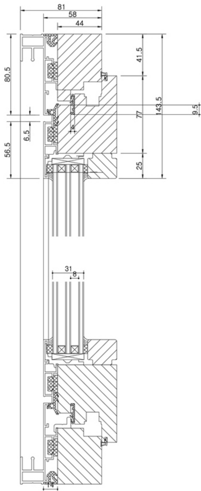
VERTICAL SECTION (A-A')
