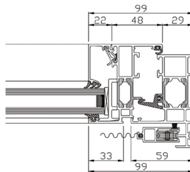
<< HORIZONTAL SECTION B-B' >>
