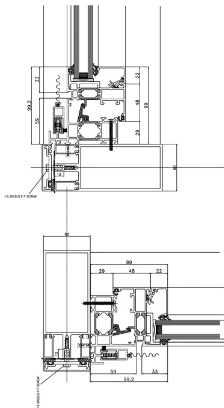
VERTICAL SECTION (A-A')
