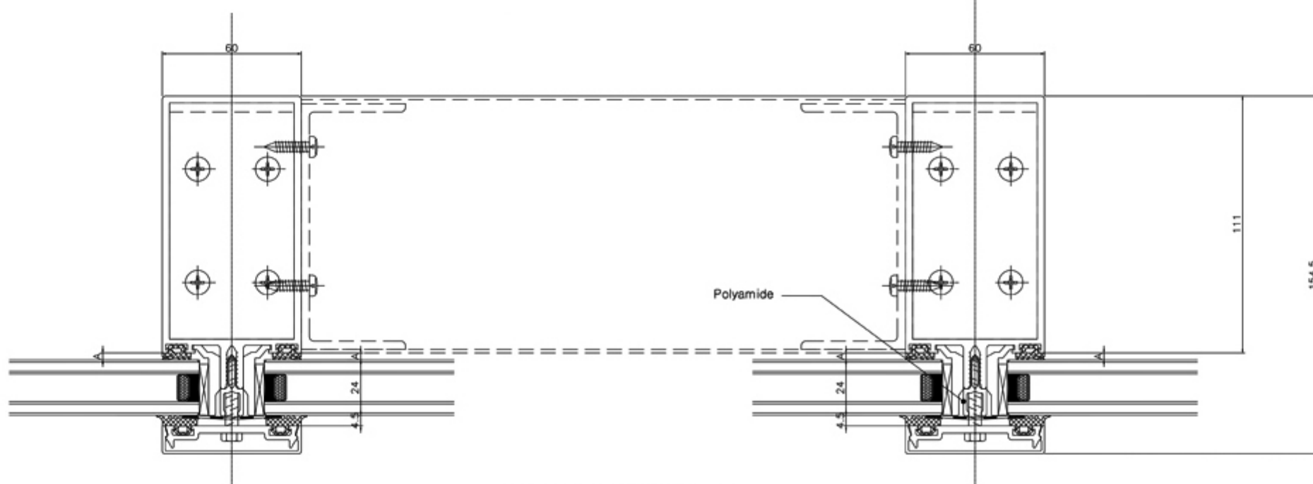
VERTICAL SECTION (B-B')
