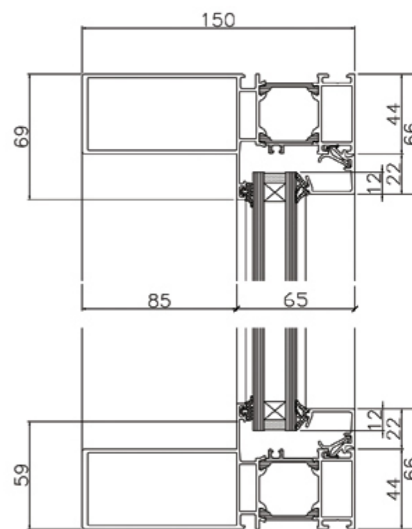
VERTICAL SECTION (B-B')
