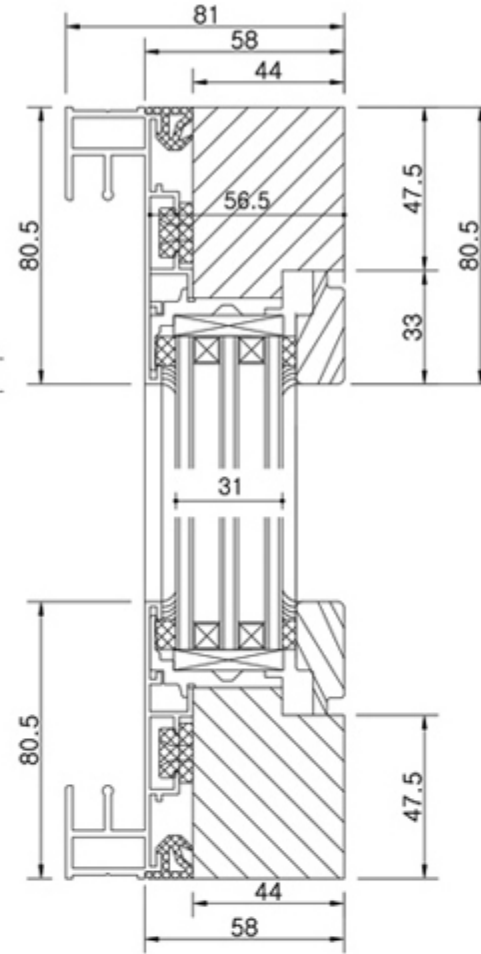
VERTICAL SECTION (B-B')
